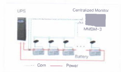
MMBM-3 Battery monitor system
